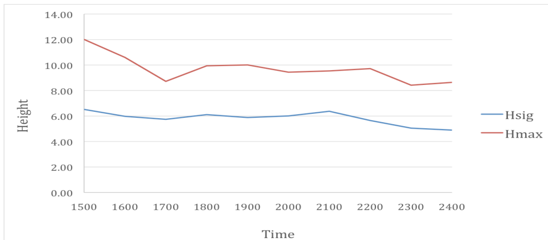
Figure 4. Data from the Sydney waverider buoy for the period of interest
