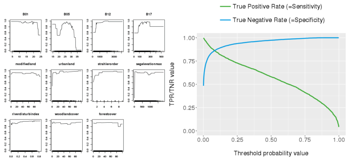
Figure 30 Response curves (left) and sensitivity-specificity plot (right)
