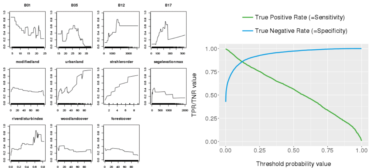
Figure 31 Response curves (left) and sensitivity-specificity plot (right)
